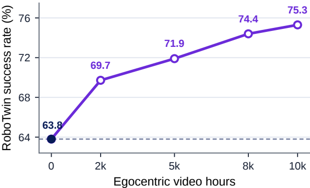
(a) Egocentric mid-training
